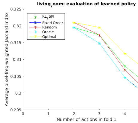
Fig. 7. Comparison of our LSPI learned policy against the Optimal Combination as well as three baselines: Fixed Order , Random Order , Oracle in the living room scene in NYUD-V2 dataset (best viewed in color). The yellow curve shows the evolution of Optimal Combination as more actions are taken into consideration. The Optimal Combination of segmentation outperforms all three baselines and our LSPI learned policy since it picks the combination that results in maximum reward for semantic segmentation.
