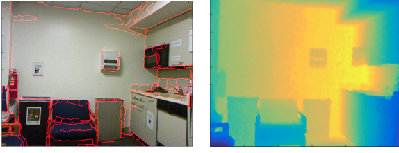
Fig. 2. Our superpixel image (bounded by red lines) and the depth image from NYUD V2. Notice how our superpixels capture the large planar surfaces.
