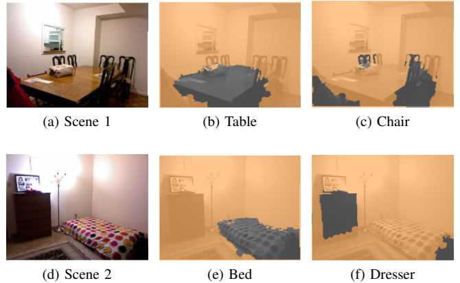
Fig. 1: Our recognition and segmentation output in the NYU V2 dataset. 1a is an example scene. The final segmentation for Table (an object of interest) is shown in 1b in gray color. If we seek for the Chair object on the same image, we get the segmentation in 1c. In 1e, 1f, we demonstrated our recognition and segmentation results for Bed , Dresser respectively for another scene.
