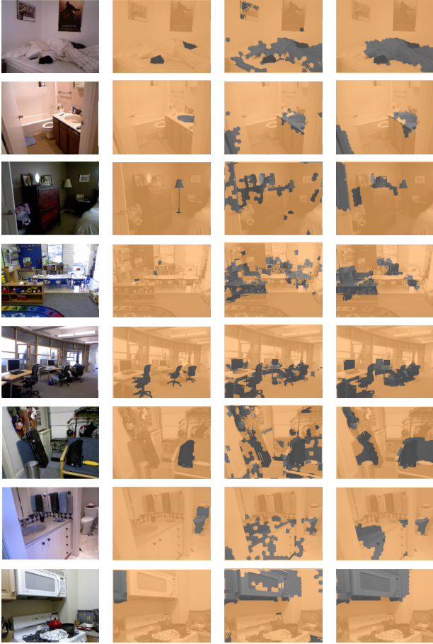
Fig. 5: The columns represent the original RGB image, ground truth, unary, and CRF output respectively from our approach in the NYU V2 dataset. Each row represents a case study for a particular object interest. From top to bottom, the objects of interest are Clothes , Sink , Lamp , Box , Chair , Bag , Toilet , and Cabinet respectively.
